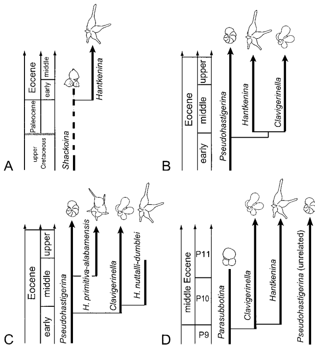
FIGURE 1. The various hypotheses on Hantkenina phylogeny. A, Hantkenina is monophyletic and evolved from Cretaceous tubulospino-se genus Shackoina (Pl. 2, Fig. 1) in the early middle Eocene (e.g. Cushman and Wickenden, 1930; Cushman, 1933; Thalmann, 1932, 1942; Rey, 1939; Brönnimann, 1950; Bolli and others, 1957). B, Hantkenina is monophyletic and evolved directly from genus Pseudohastigerina at the base of the middle Eocene (intermediates unknown), Clavigerinella is sister taxon to Hantkenina (Banner and Lowry 1985, Pearson, 1993). C, Hantkenina is polyphyletic and middle and late Eocene groups evolved independently from different pseudohastigerinid ancestors (Blow and Banner, 1962; and Blow, 1979; Berggren and others, 1967). Stellate early middle Eocene forms are linked to the proposed ancestor Pseudohastigerina via intermediate morphotype Clavigerinella , which is considered sister taxon to Hantkenina . A similar relationship was proposed by Dieni and Proto Decima (1964) and Steineck (1971). D, Hantkenina is monophyletic. It evolved from Clavigerinella and is unrelated to Pseudohastigerina (Shackina, 1937; Benjamini and Reiss, 1979; this study).
