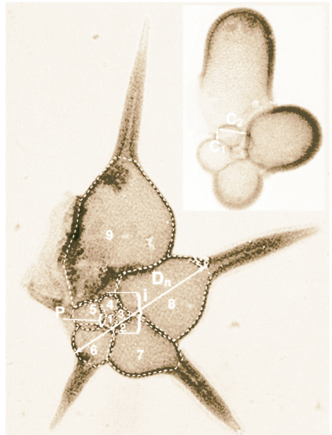
FIGURE 3. Morphometric variables measured from X-rays. The dashed line traces the perimeter of each chamber. U, number of chambers in the ultimate whorl = 'whole number of chambers in ultimate whorl' + [C1/(C1+C2)] . D_n = maximum test diameter at chamber n, i = initial whorl, P = proloculus (= chamber 1 ).
